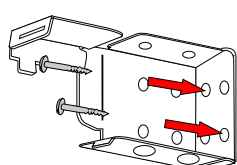
Face-Fixing: Where the bracket is fixed onto the wall or straight onto the window frame.
