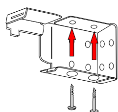
Top-Fixing: Where the bracket will be fixed directly to the ceiling or underside of the recess.
