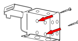
Side-Fixing: Where the bracket is fixed on the side wall of a recess.
