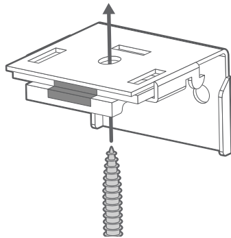
Top-Fixing
