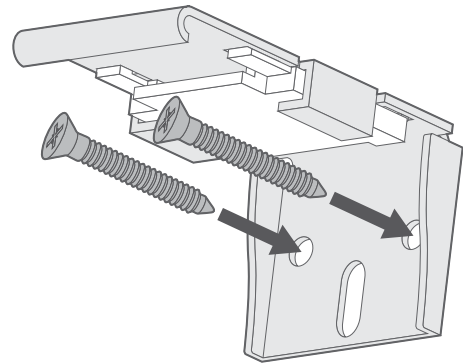
Face-Fixing
