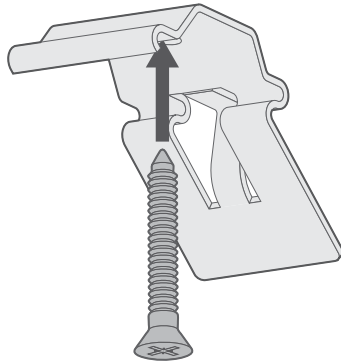
Top-Fixing
